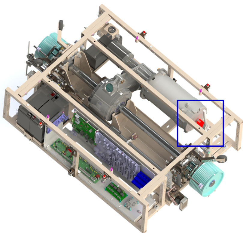
Figure 10: Manual Lowering Ratchet
