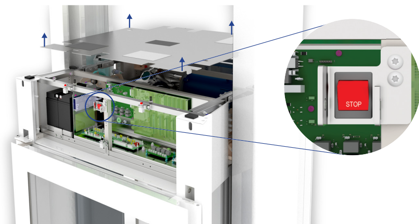
Figure 8: Top cover and controller switch
